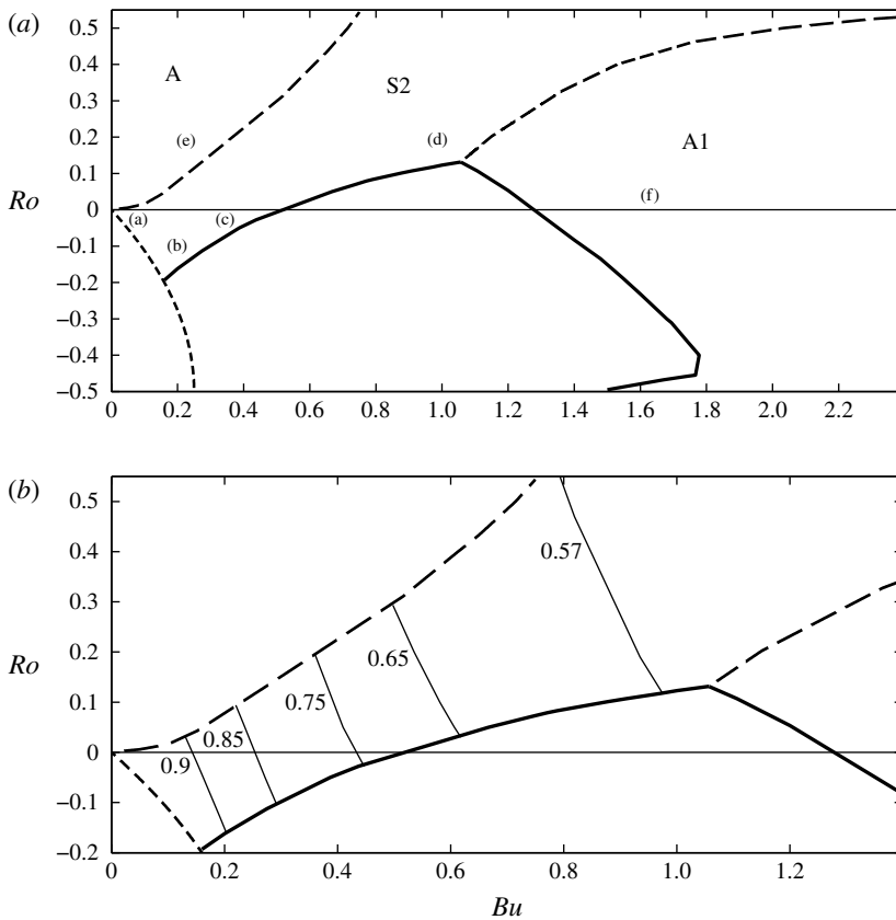
FIGURE 13. Panel (a) shows a simplification of the parameter map in figure 8(a). The fastest-growing eigenmodes in the region labelled A are antisymmetric in z and have azimuthal wavenumbers of 1, 2, 3 or 4; otherwise, the fastest-growing eigenmodes have the symmetry of the large labels. The small labels (a)–(f) indicate the locations in parameter space of the vortices whose fastest-growing eigenmodes are plotted in figure 14. Panel (b) shows a blow up of the S2 region in panel (a). The thin solid curves are the iso-contours of the enstrophy S_{shield} of the vertical vorticity of the eigenmode in the vortex shield. The value of S_{shield} in the S2 region decreases from 0.95 to 0.55 with increasing Bu . The approximate average value of S_{core} in the A and A1 regions are 0.95 and 0.73, respectively. In the lower left corner of panel (a) where N_c^2 < 0 , S_{core} \simeq 0.99 .
