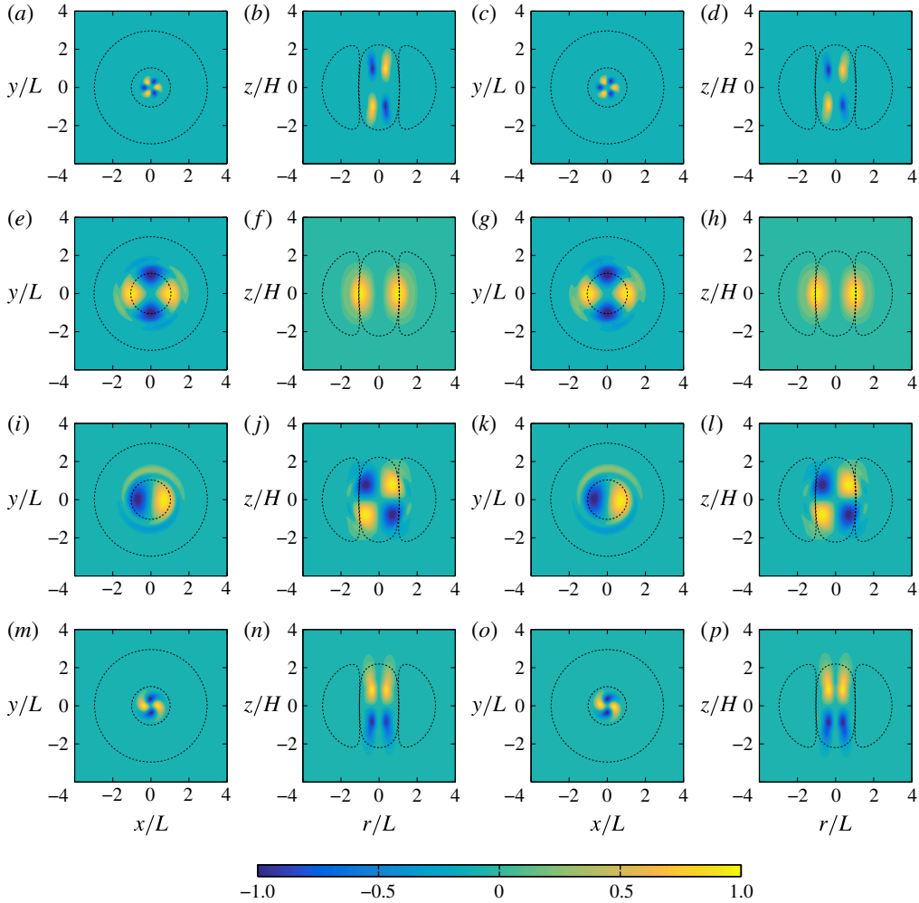
FIGURE 12. (Colour online) Vertical vorticity of eigenmodes normalized such that the maximum value of |\omega| is 1. The eigenmodes are virtually indistinguishable for f/\bar{N}=0.1 and f/\bar{N}=0.01 . The four rows from top to bottom correspond to the first four rows in table 1. The broken lines denote the boundaries of the core and shield of the unperturbed Gaussian vortex. Panels (a,b,e,f,i,j,m,n) are for f/\bar{N}=0.1 and (c,d,g,h,k,l,o,p) are for f/\bar{N}=0.01 . Panels (a,c,e,g,i,k,m,o) show the eigenmodes in the x - y plane for a fixed z . For the z -symmetric eigenmode in the second row, this fixed value is z=0 . For the antisymmetric eigenmodes in rows 1, 3 and 4, the fixed value of z is the positive value of z at which |\omega| of the eigenmode obtains its maximum value. Panels (b,d,f,h,j,l,n,p) show the eigenmodes in the r - z plane for fixed azimuthal angle \phi . In all cases, \phi is chosen so that it is the angle at which \omega of the eigenmode obtains its maximum value.
